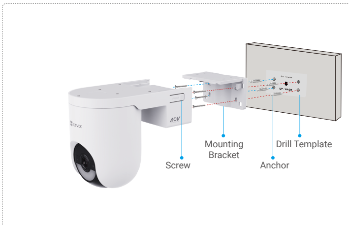
Fig. 2 Wall Mount
